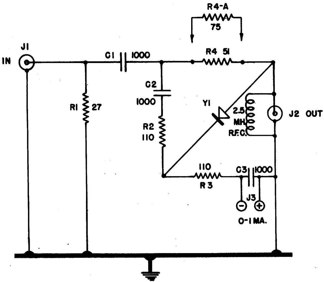
SCHEMATIC CIRCUIT DIAGRAM
